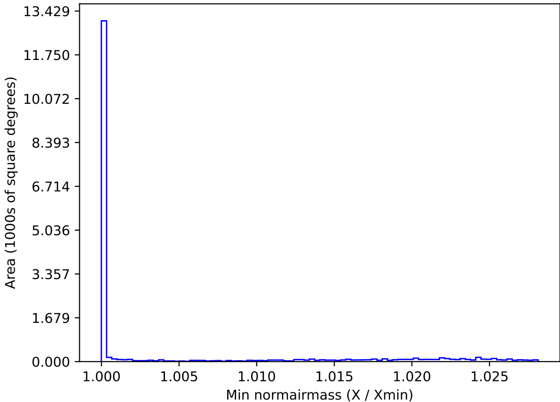
too_elab_r16_d3_gz_v3.4_10yrs WFD all bands: Min normairmass
