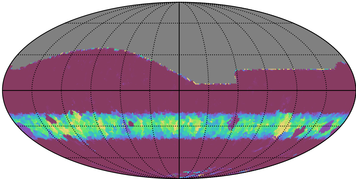
too_elab_r16_d3_gz_v3.4_10yrs All sky g band: Min normairmass
