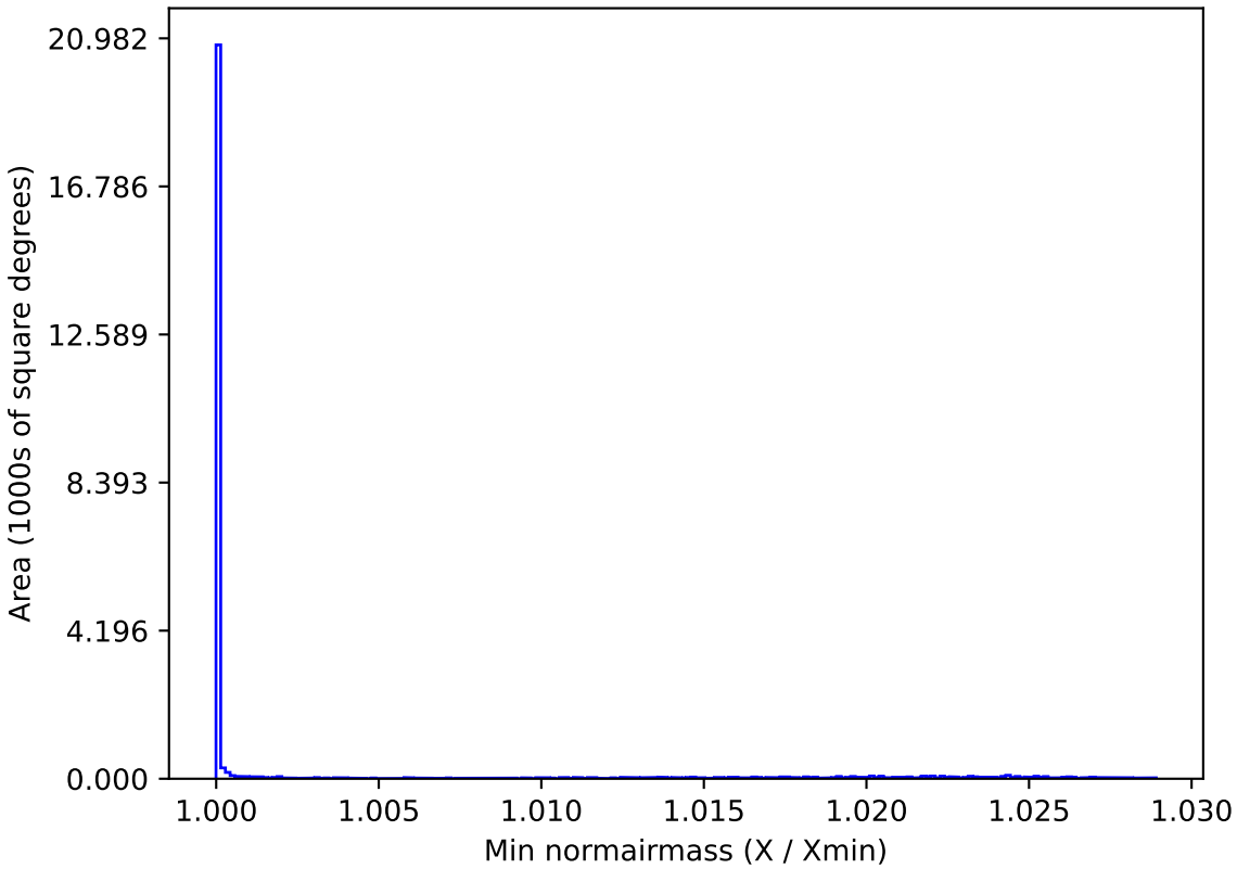
too_elab_r16_d3_gz_v3.4_10yrs All sky all bands: Min normairmass
