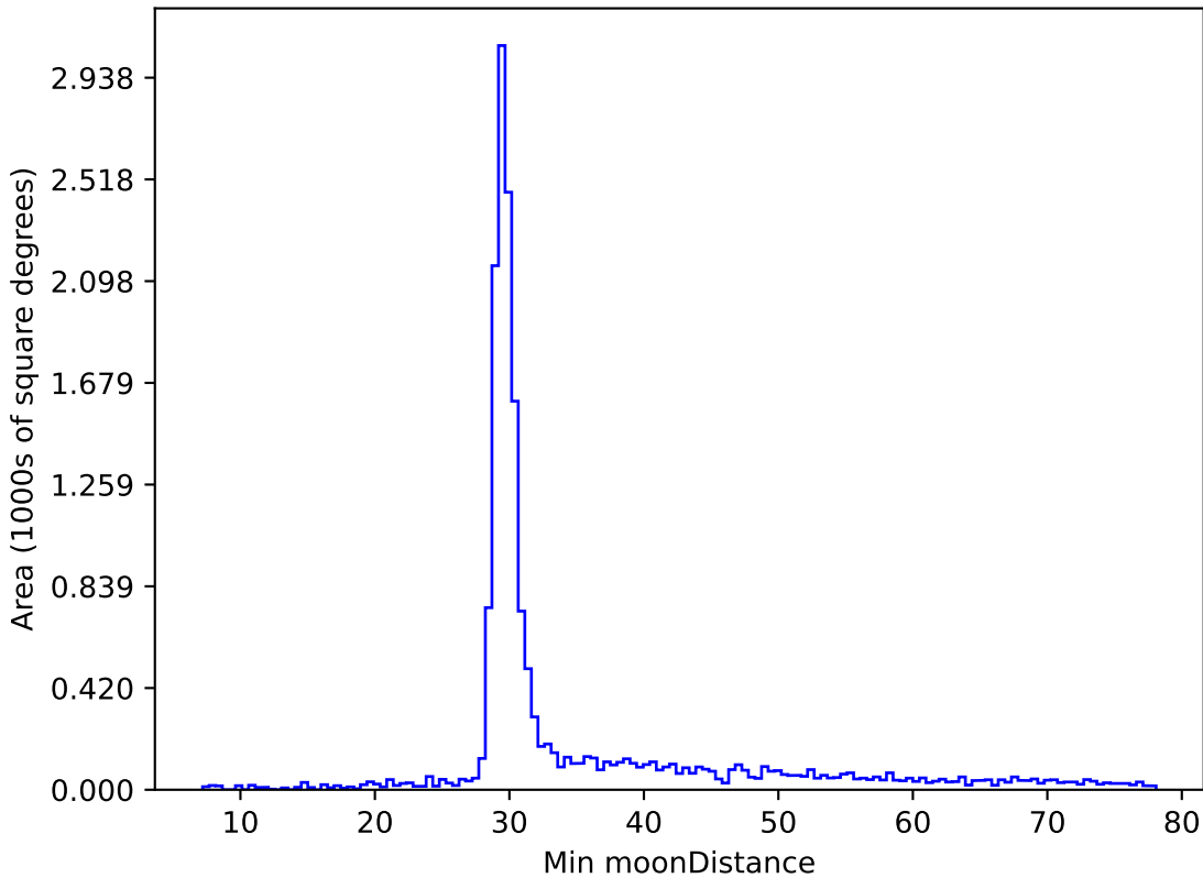
too_elab_r16_d3_gz_v3.4_10yrs WFD z band: Min moonDistance
