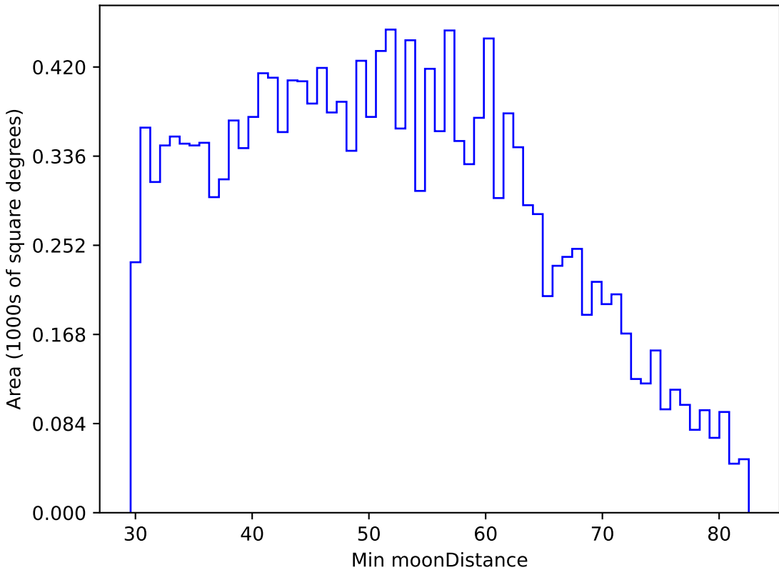
too_elab_r16_d3_gz_v3.4_10yrs WFD u band: Min moonDistance
