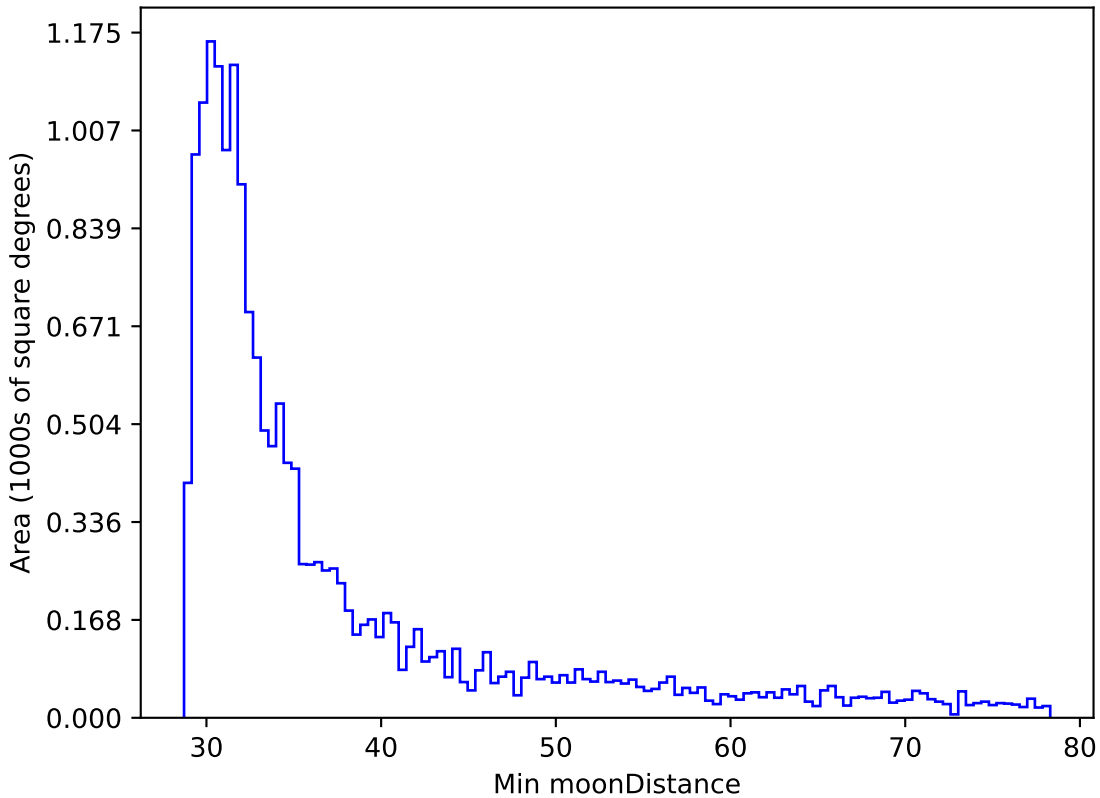
too_elab_r16_d3_gz_v3.4_10yrs WFD r band: Min moonDistance
