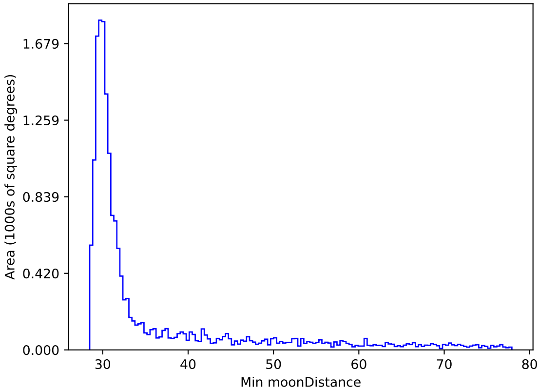
too_elab_r16_d3_gz_v3.4_10yrs WFD i band: Min moonDistance
