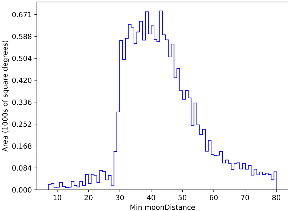
too_elab_r16_d3_gz_v3.4_10yrs WFD g band: Min moonDistance
