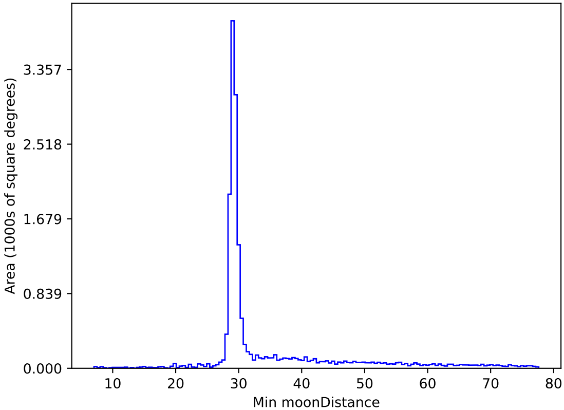
too_elab_r16_d3_gz_v3.4_10yrs WFD all bands: Min moonDistance
