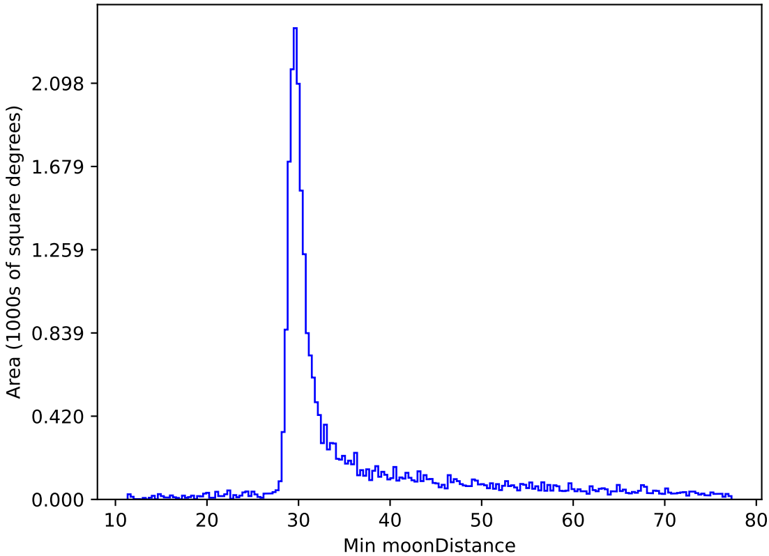
too_elab_r16_d3_gz_v3.4_10yrs All sky z band: Min moonDistance
