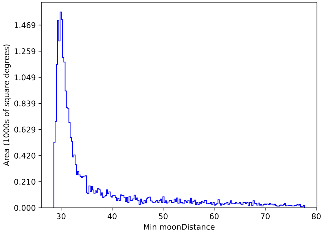
too_elab_r16_d3_gz_v3.4_10yrs All sky i band: Min moonDistance
