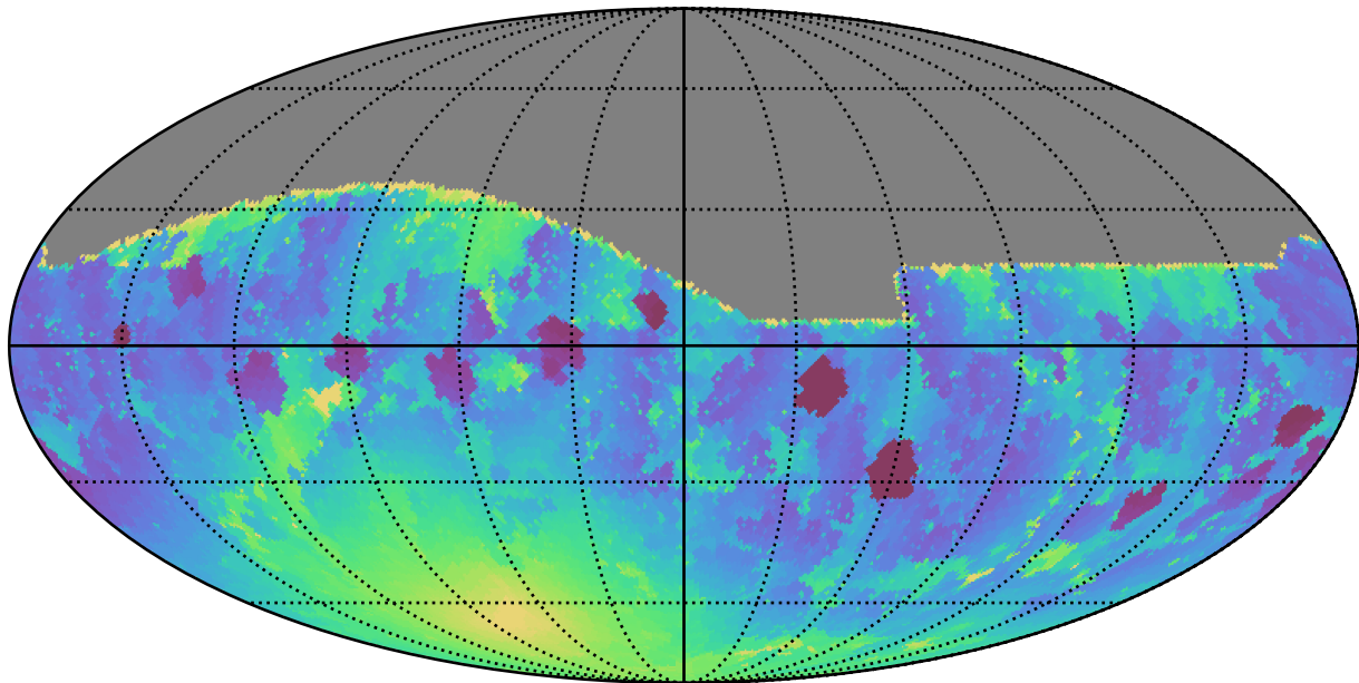
too_elab_r16_d3_gz_v3.4_10yrs All sky g band: Min moonDistance
