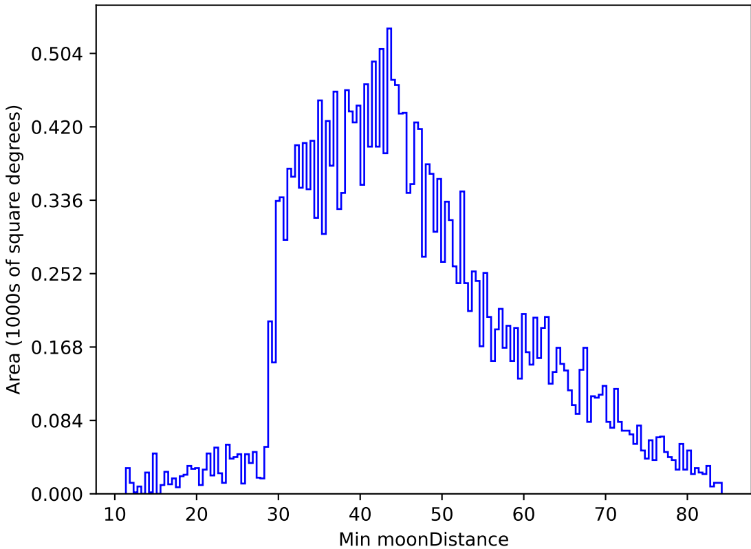
too_elab_r16_d3_gz_v3.4_10yrs All sky g band: Min moonDistance
