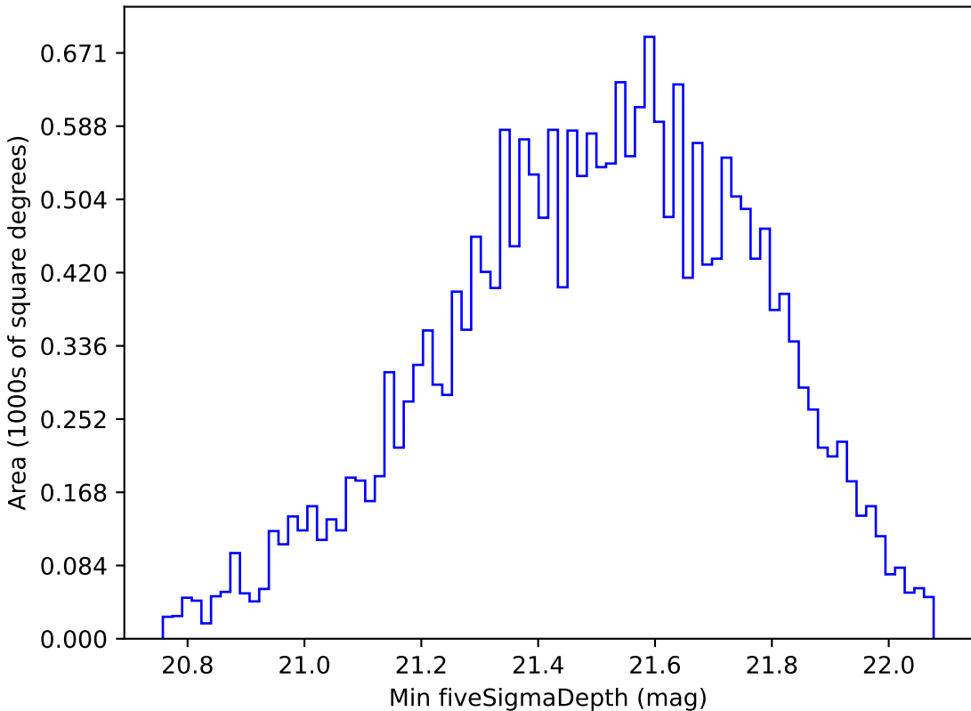
too_elab_r16_d3_gz_v3.4_10yrs Yr 1 y band: Min fiveSigmaDepth
