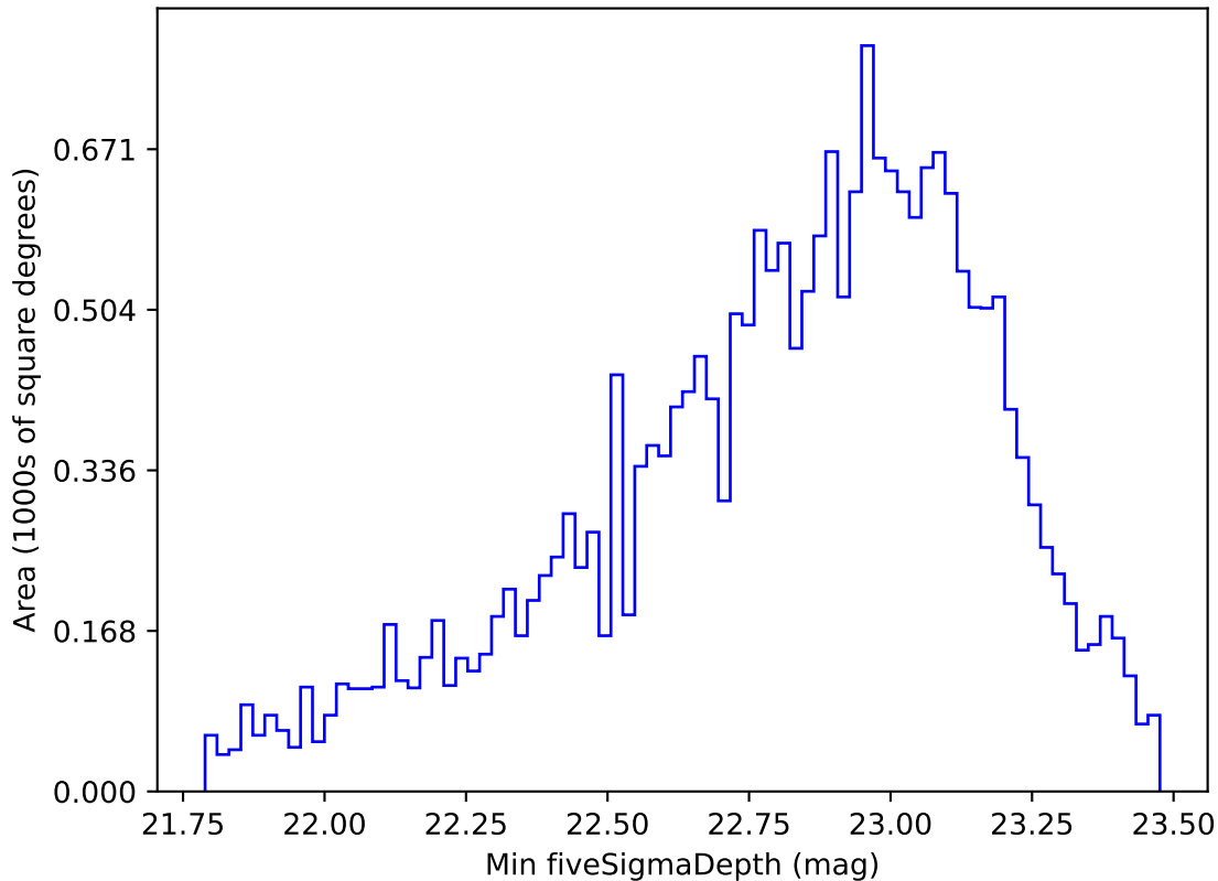
too_elab_r16_d3_gz_v3.4_10yrs Yr 1 u band: Min fiveSigmaDepth
