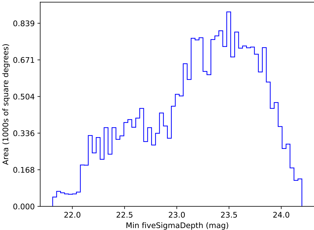
too_elab_r16_d3_gz_v3.4_10yrs Yr 1 r band: Min fiveSigmaDepth
