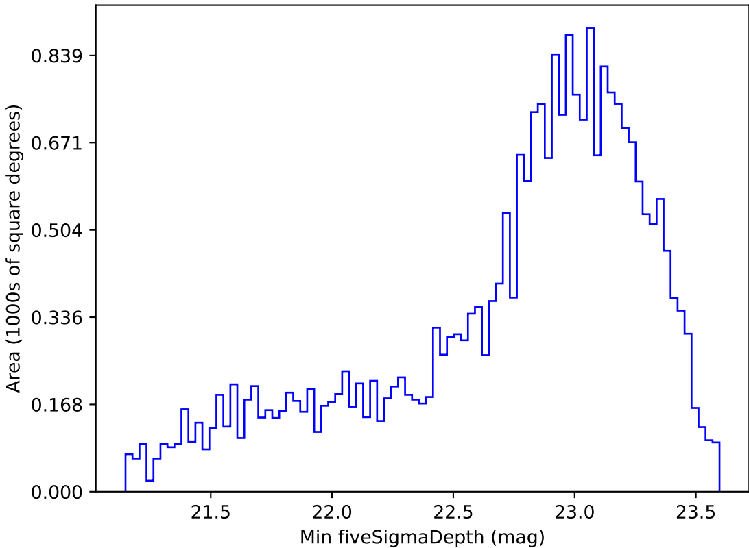
too_elab_r16_d3_gz_v3.4_10yrs Yr 1 i band: Min fiveSigmaDepth
