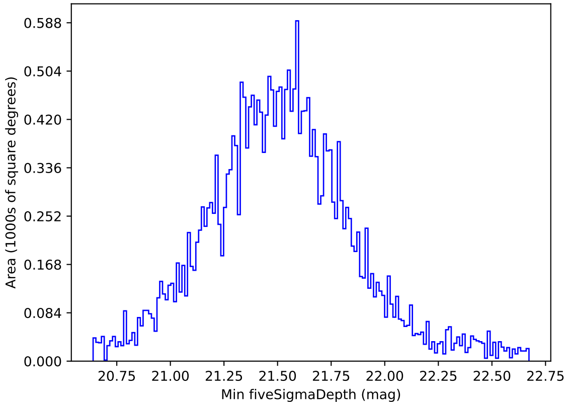
too_elab_r16_d3_gz_v3.4_10yrs Yr 1 all bands: Min fiveSigmaDepth
