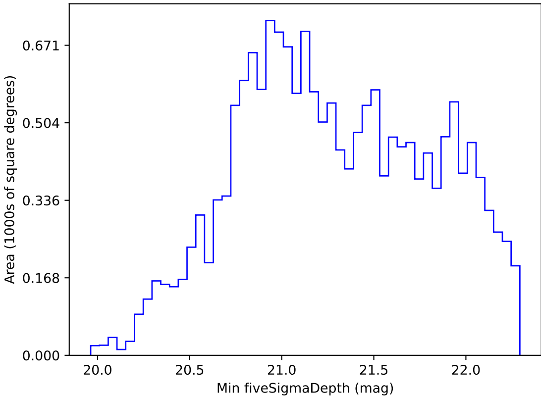
too_elab_r16_d3_gz_v3.4_10yrs WFD z band: Min fiveSigmaDepth
