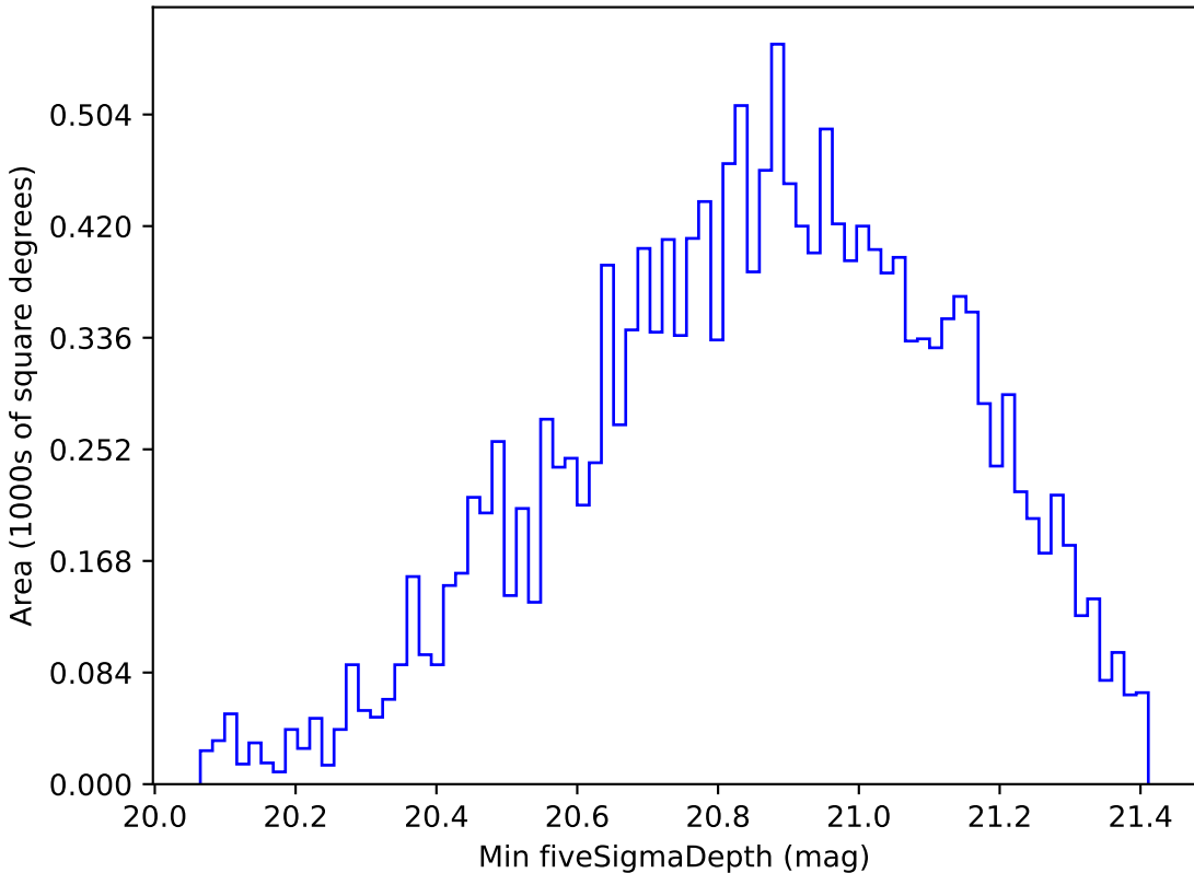
too_elab_r16_d3_gz_v3.4_10yrs WFD y band: Min fiveSigmaDepth
