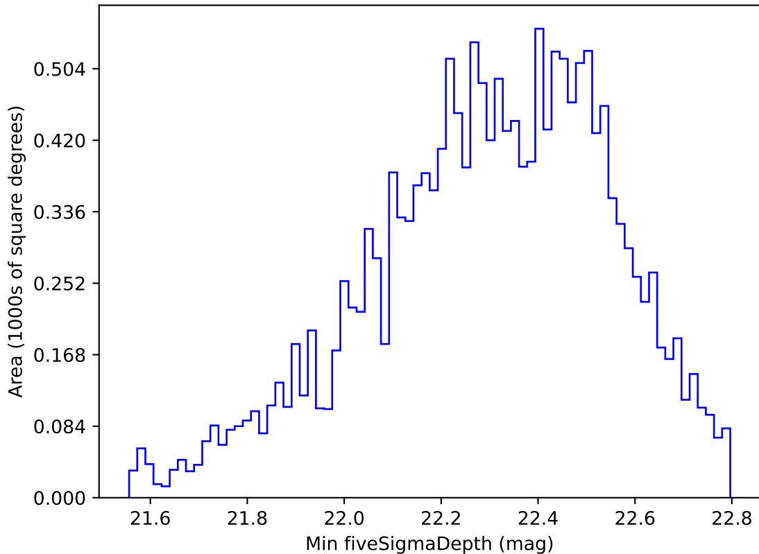
too_elab_r16_d3_gz_v3.4_10yrs WFD u band: Min fiveSigmaDepth
