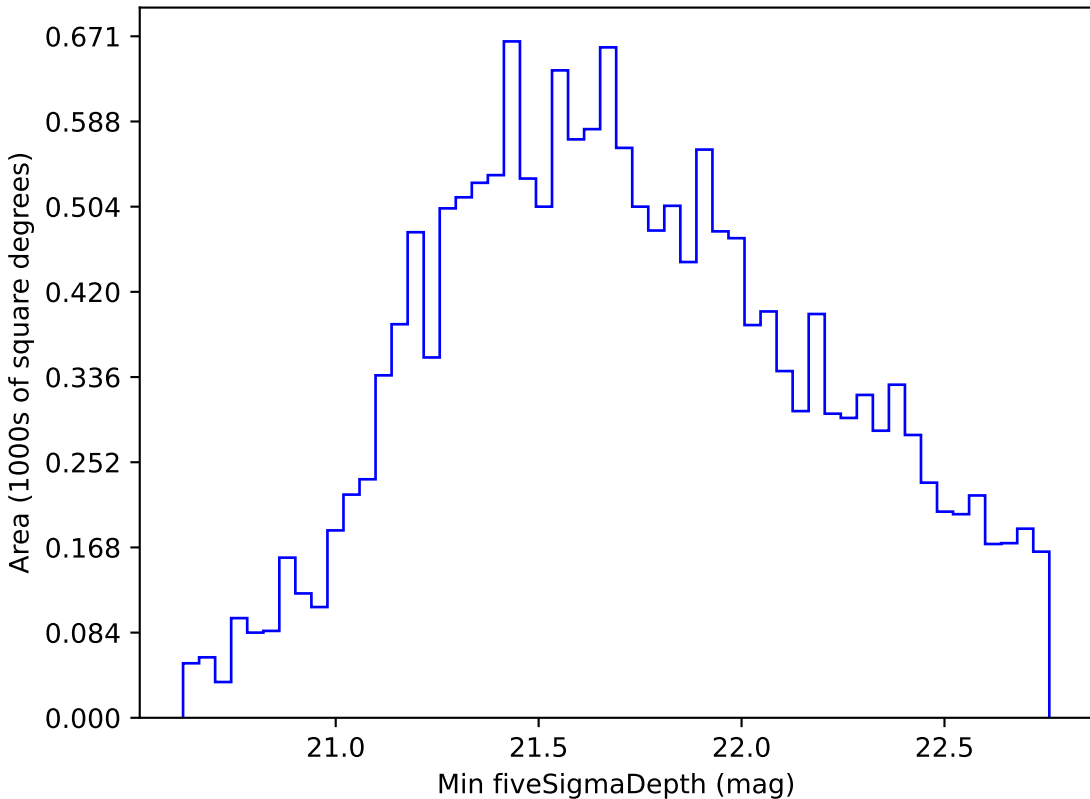
too_elab_r16_d3_gz_v3.4_10yrs WFD i band: Min fiveSigmaDepth
