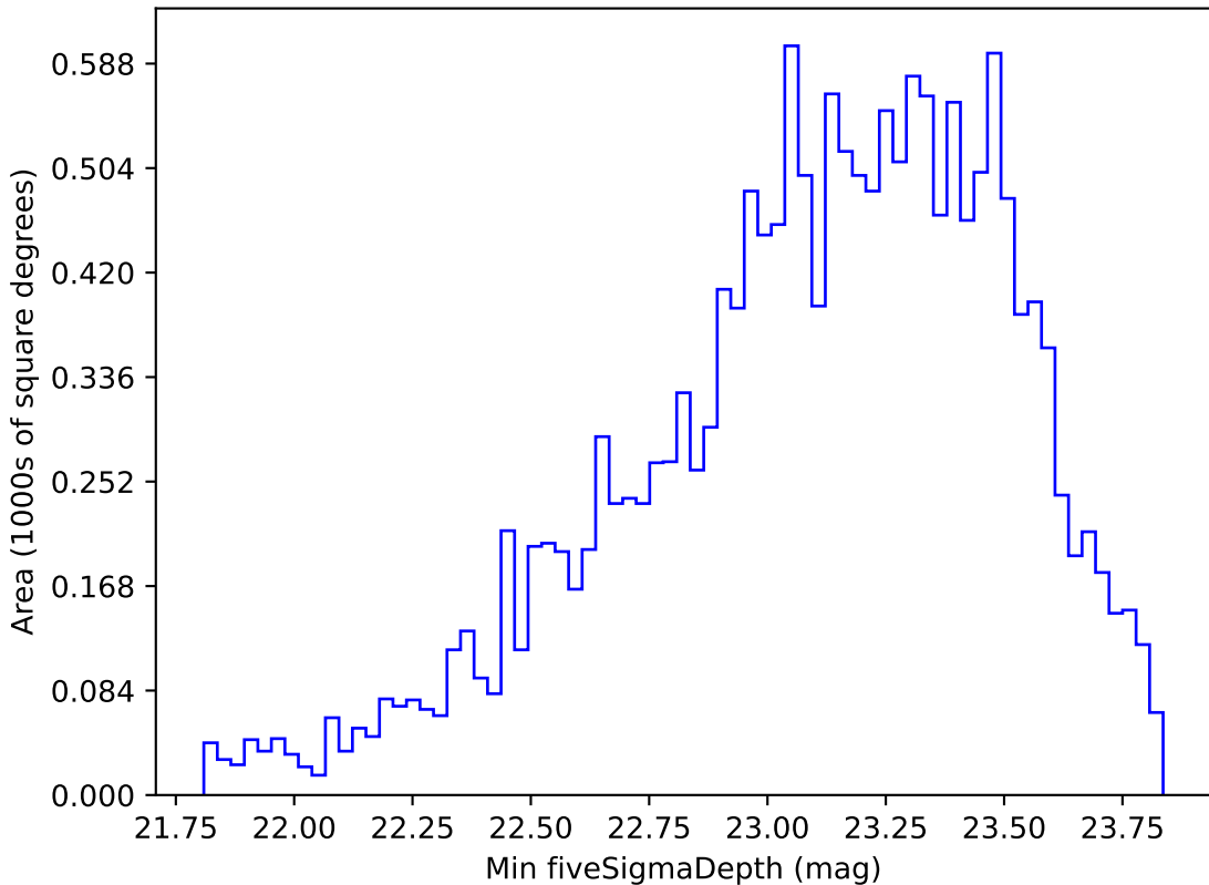
too_elab_r16_d3_gz_v3.4_10yrs WFD g band: Min fiveSigmaDepth
