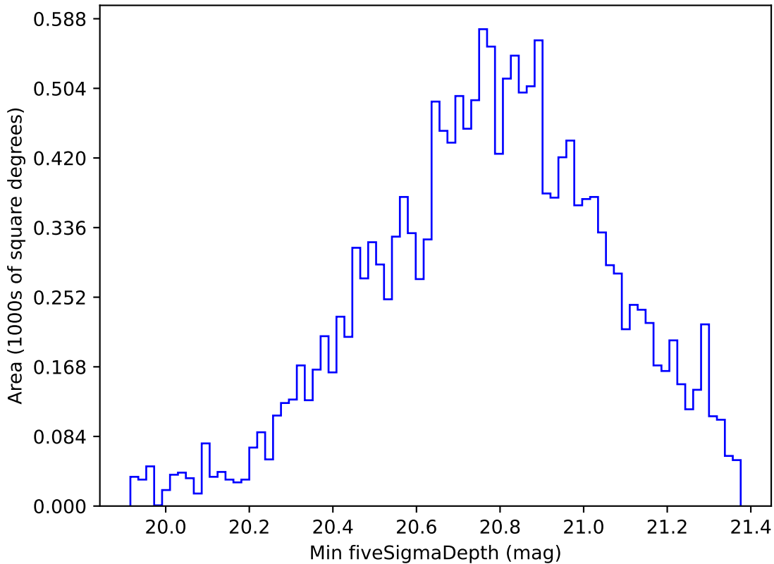
too_elab_r16_d3_gz_v3.4_10yrs WFD all bands: Min fiveSigmaDepth
