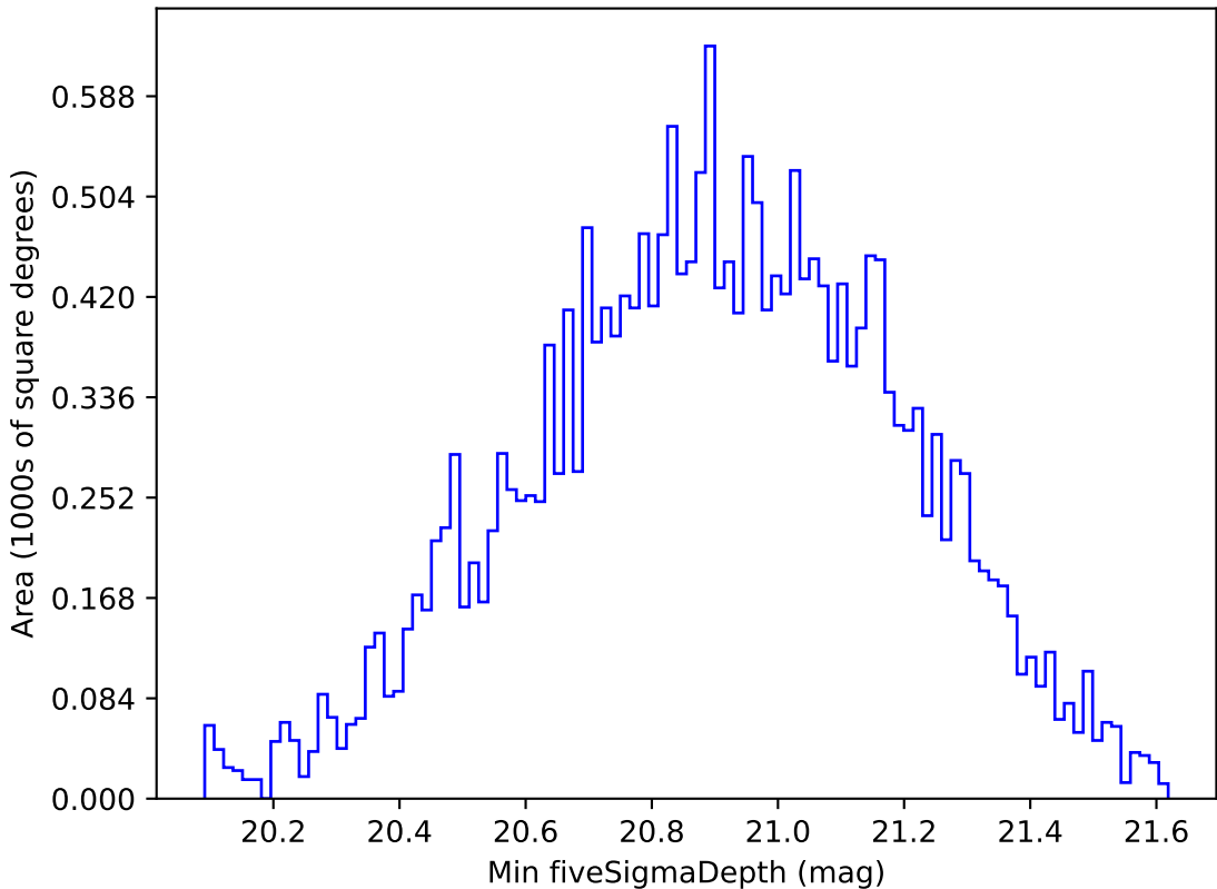
too_elab_r16_d3_gz_v3.4_10yrs All sky y band: Min fiveSigmaDepth
