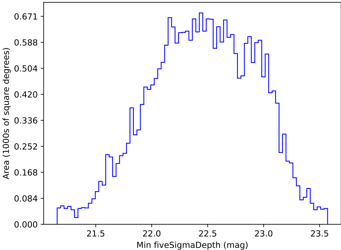
too_elab_r16_d3_gz_v3.4_10yrs All sky r band: Min fiveSigmaDepth
