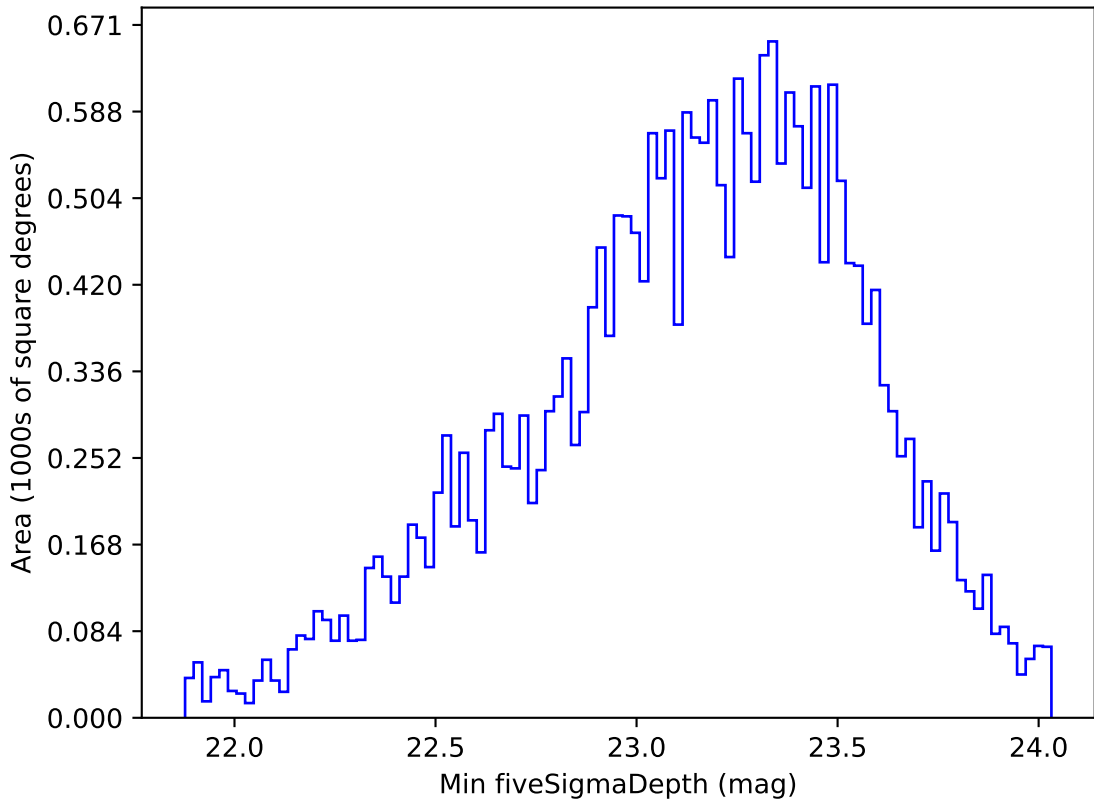
too_elab_r16_d3_gz_v3.4_10yrs All sky g band: Min fiveSigmaDepth
