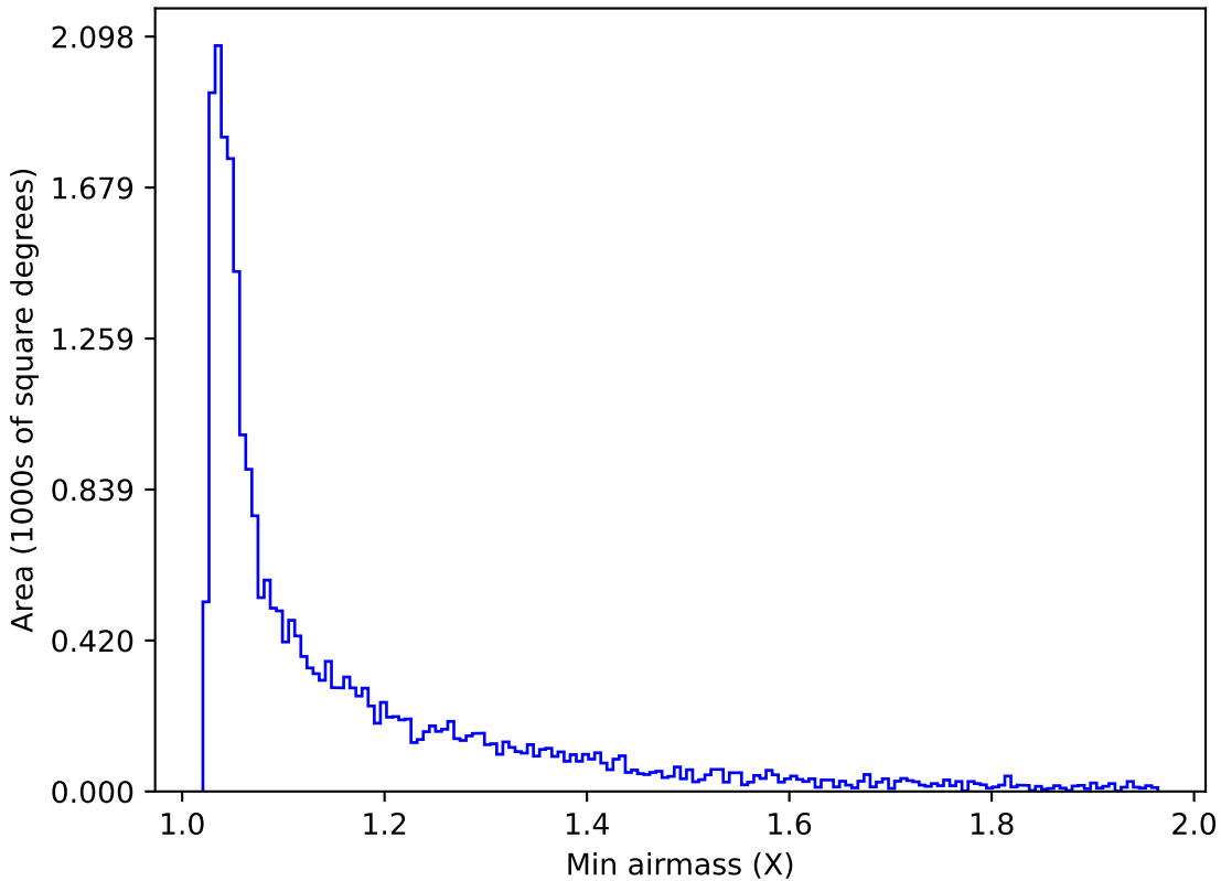
too_elab_r16_d3_gz_v3.4_10yrs Yr 1 z band: Min airmass
