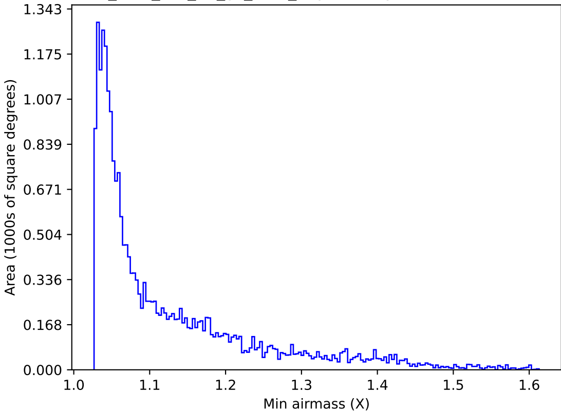
too_elab_r16_d3_gz_v3.4_10yrs Yr 1 y band: Min airmass
