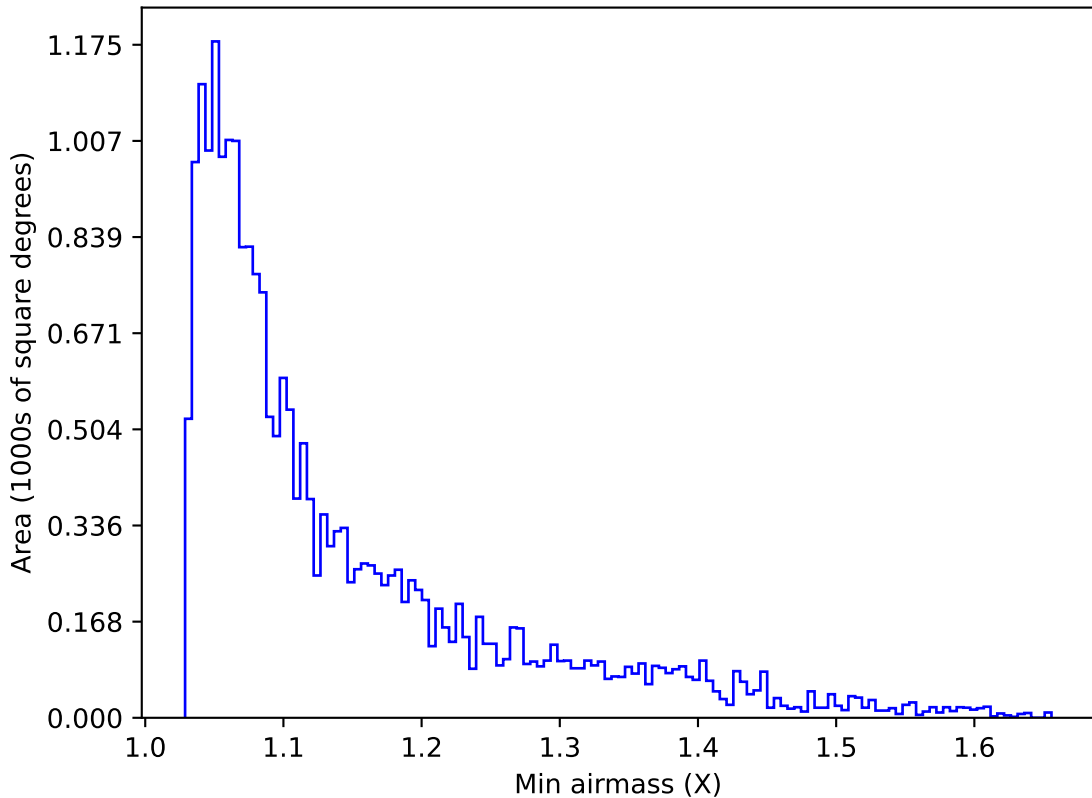
too_elab_r16_d3_gz_v3.4_10yrs Yr 1 u band: Min airmass
