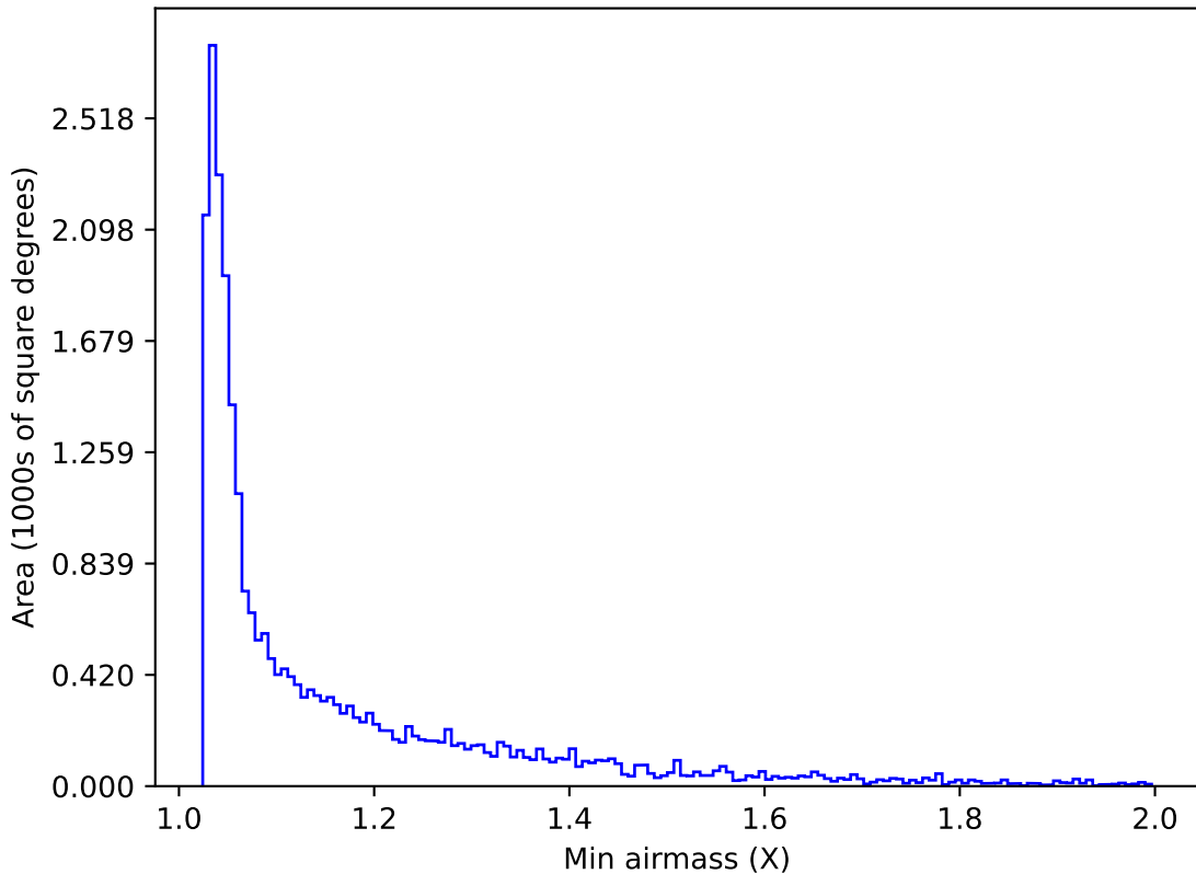
too_elab_r16_d3_gz_v3.4_10yrs Yr 1 r band: Min airmass
