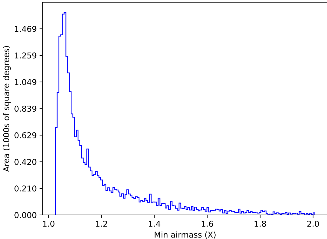
too_elab_r16_d3_gz_v3.4_10yrs Yr 1 g band: Min airmass
