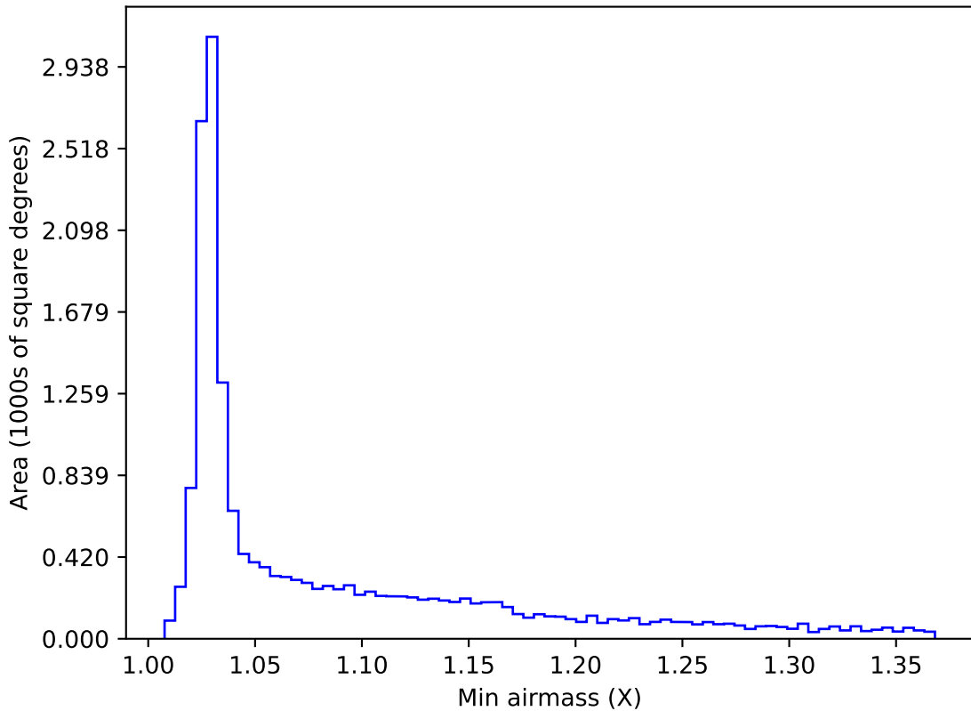
too_elab_r16_d3_gz_v3.4_10yrs WFD z band: Min airmass
