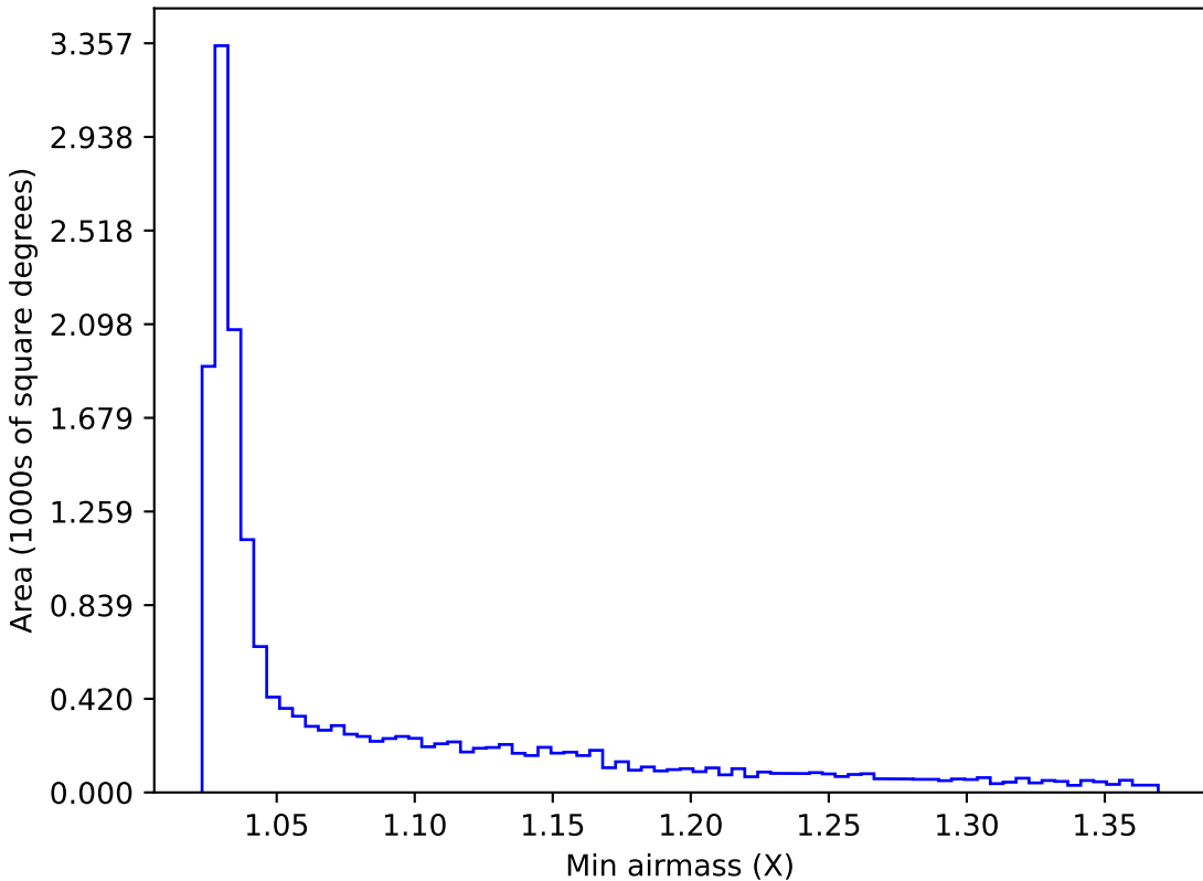
too_elab_r16_d3_gz_v3.4_10yrs WFD y band: Min airmass
