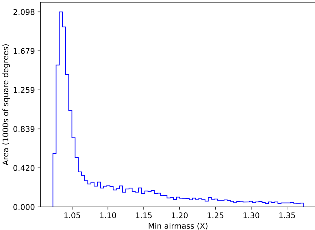
too_elab_r16_d3_gz_v3.4_10yrs WFD u band: Min airmass
