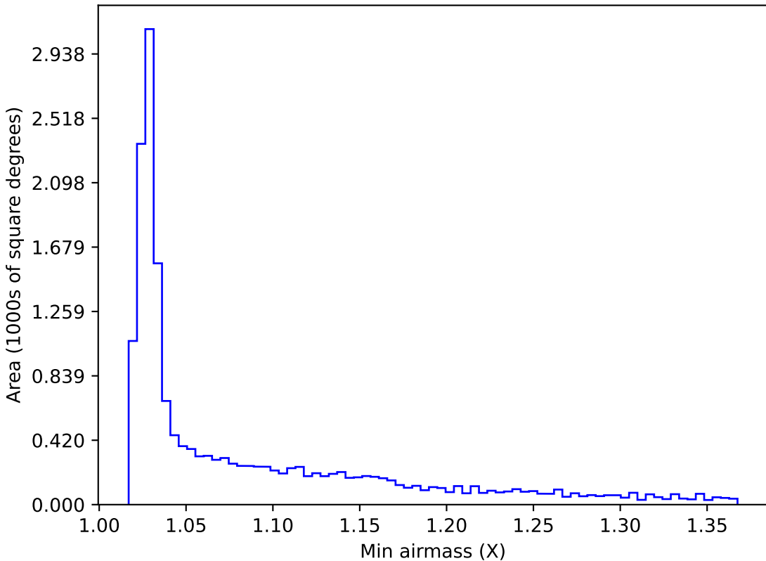
too_elab_r16_d3_gz_v3.4_10yrs WFD r band: Min airmass
