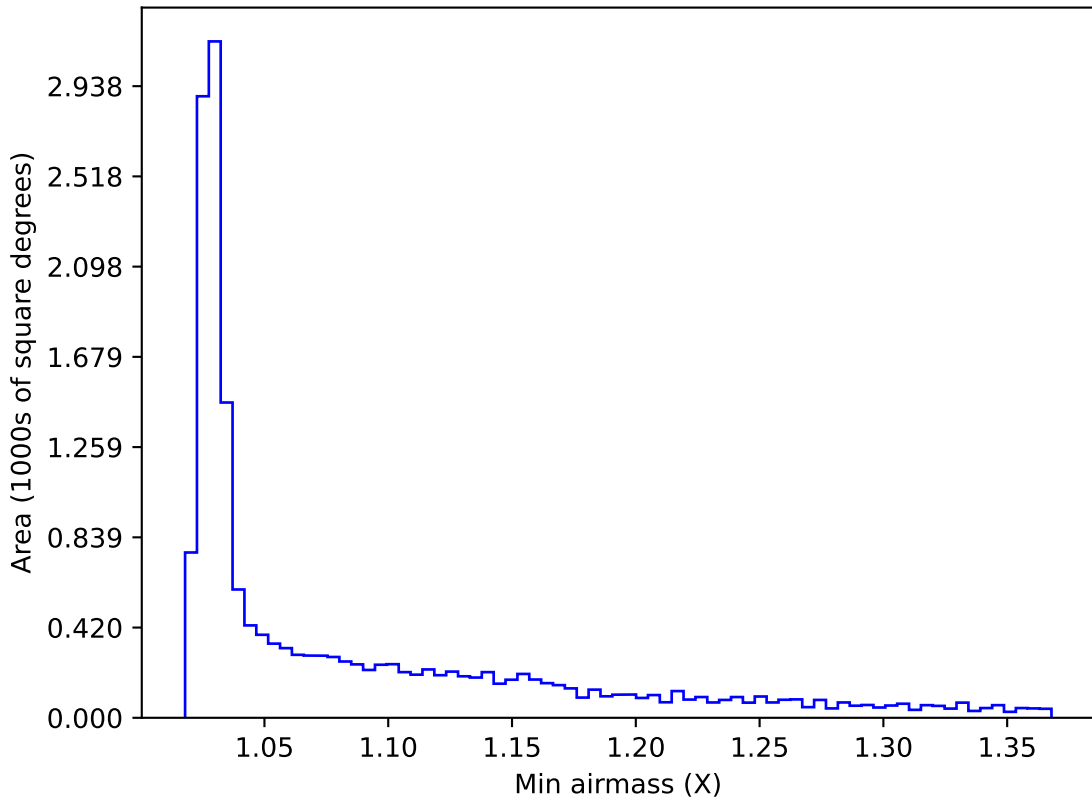
too_elab_r16_d3_gz_v3.4_10yrs WFD i band: Min airmass
