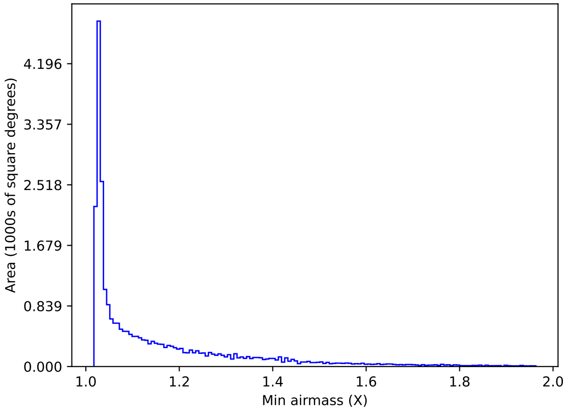
too_elab_r16_d3_gz_v3.4_10yrs All sky r band: Min airmass
