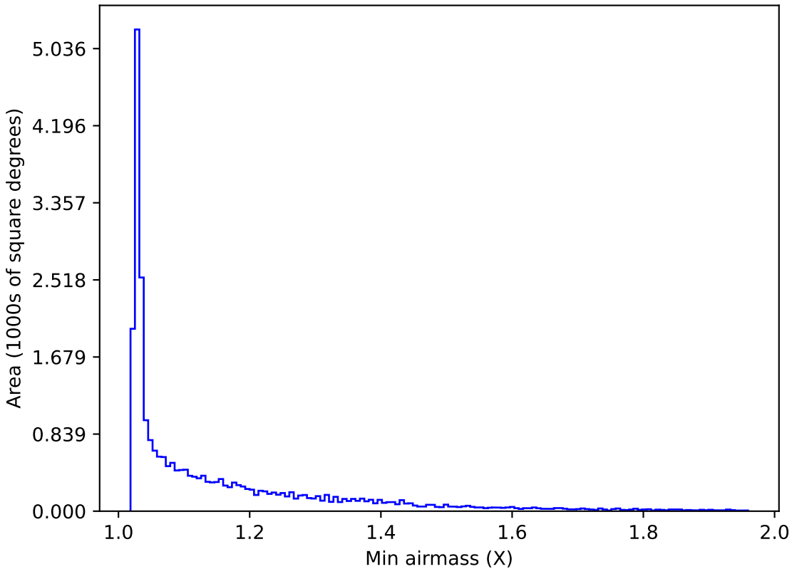
too_elab_r16_d3_gz_v3.4_10yrs All sky i band: Min airmass
