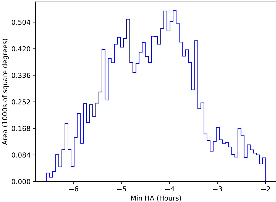
too_elab_r16_d3_gz_v3.4_10yrs WFD z band: Min HA
