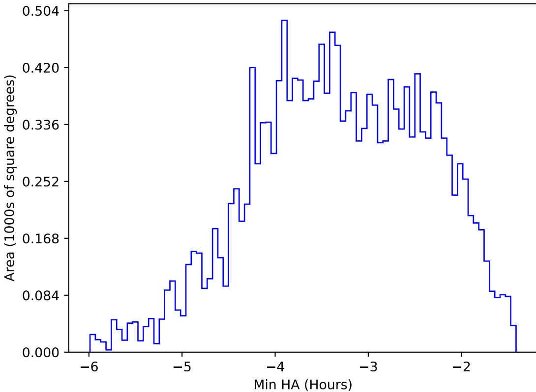
too_elab_r16_d3_gz_v3.4_10yrs WFD u band: Min HA
