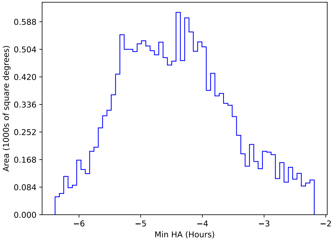
too_elab_r16_d3_gz_v3.4_10yrs WFD r band: Min HA
