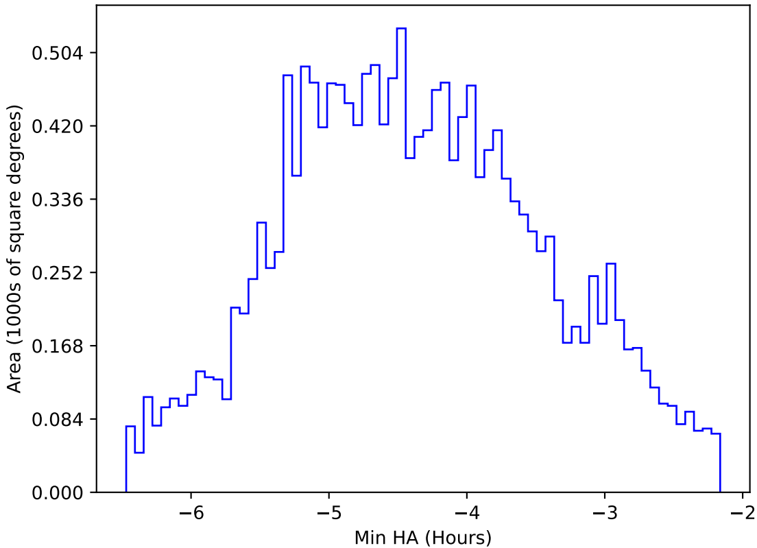
too_elab_r16_d3_gz_v3.4_10yrs WFD i band: Min HA
