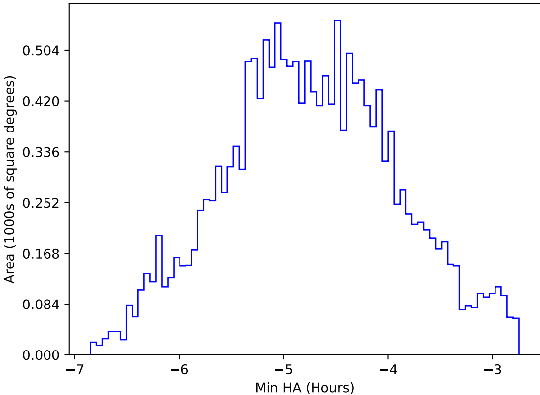
too_elab_r16_d3_gz_v3.4_10yrs WFD all bands: Min HA
