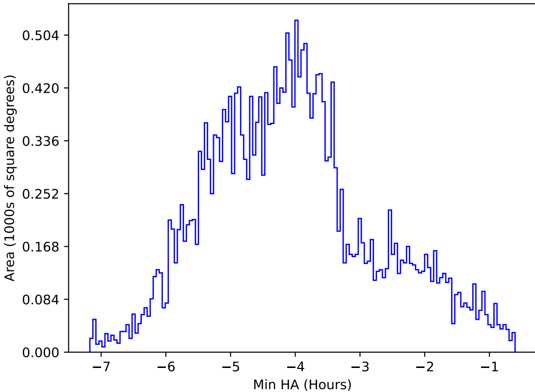
too_elab_r16_d3_gz_v3.4_10yrs All sky z band: Min HA
