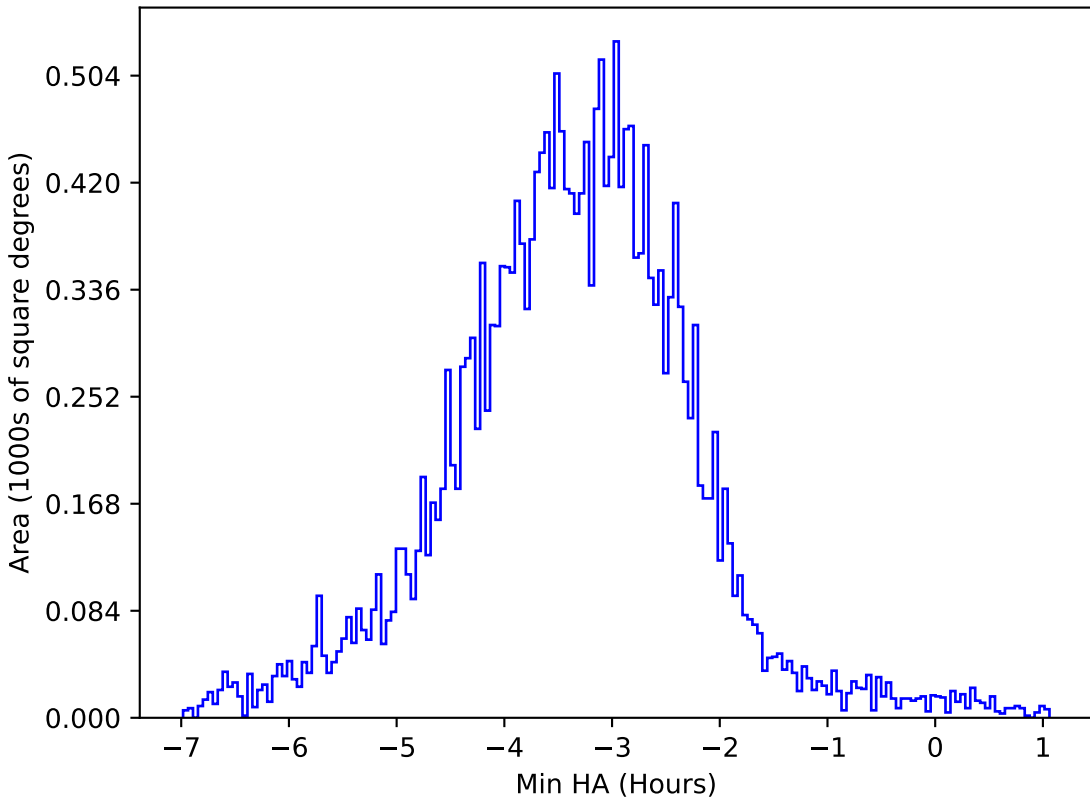
too_elab_r16_d3_gz_v3.4_10yrs All sky y band: Min HA
