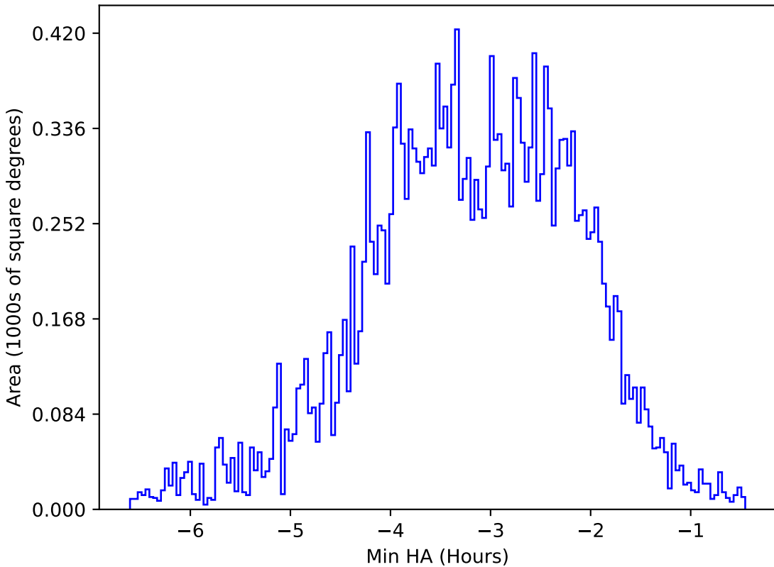
too_elab_r16_d3_gz_v3.4_10yrs All sky u band: Min HA
