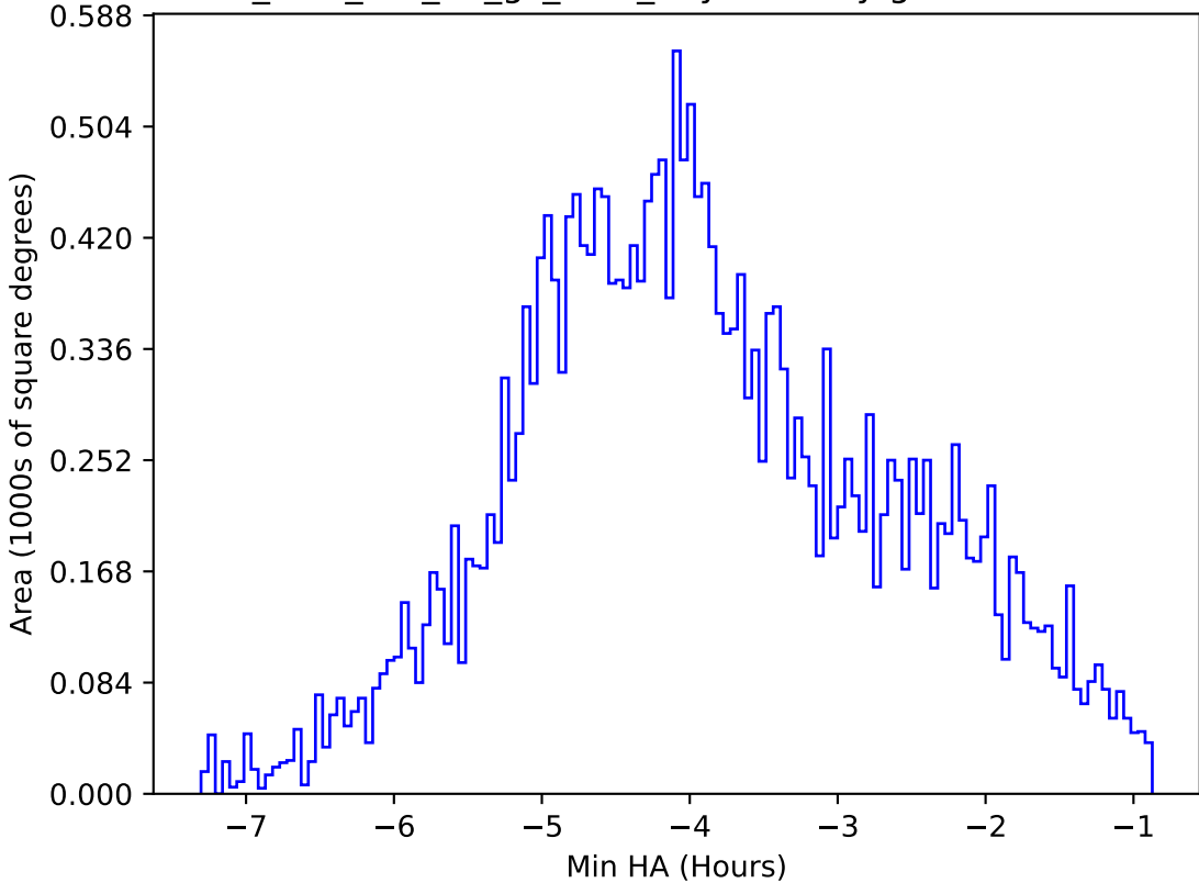
too_elab_r16_d3_gz_v3.4_10yrs All sky g band: Min HA
