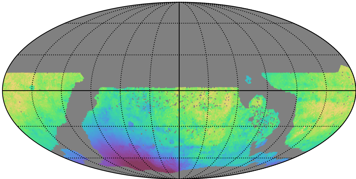
too_elab_r16_d3_gz_v3.4_10yrs WFD z band: Median solarElong
