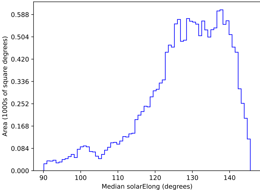
too_elab_r16_d3_gz_v3.4_10yrs WFD z band: Median solarElong
